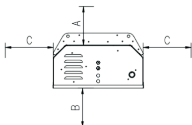
0° Mounting Angle
